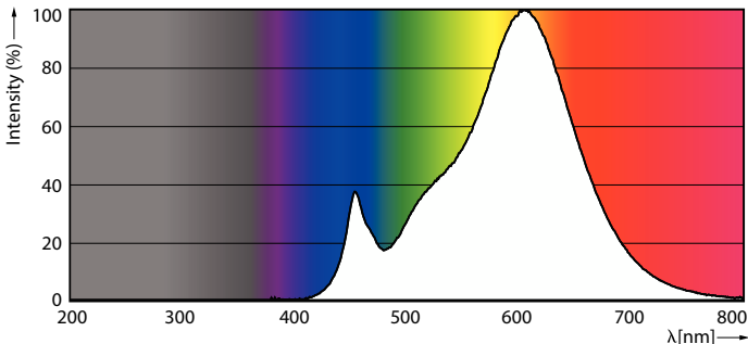
Spectral Power Distribution Colour - LEDbulb ND 4.9-40W A60 E27 827 2CT
