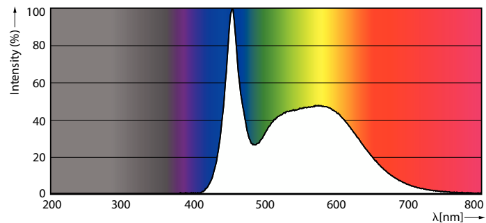
Spectral Power Distribution Colour - CorePro LEDbulb ND 4.9-40W A60 E27 865
