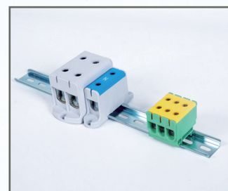
Installation on the rail
