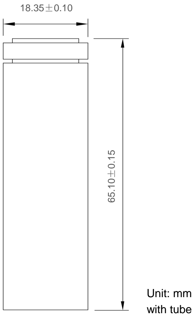
Fig. 1. Outline Dimensions of INR18650/35V
