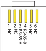
RJ11(6P2C) regulatora
