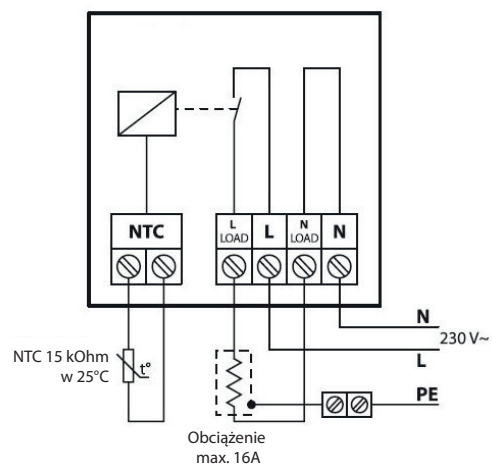
Schemat DEVlreg™ Basic
