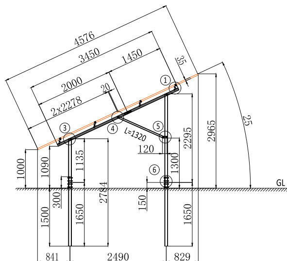
FS-Support 25°-2P Side View Scale 1:1
