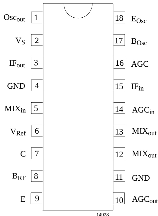
Figure 2. Pinning DIP18
