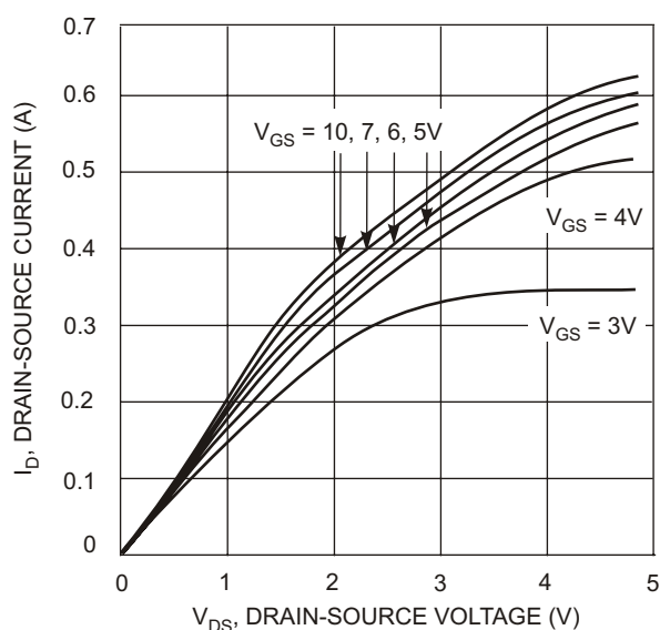
Fig. 1 On-Region Characteristics
