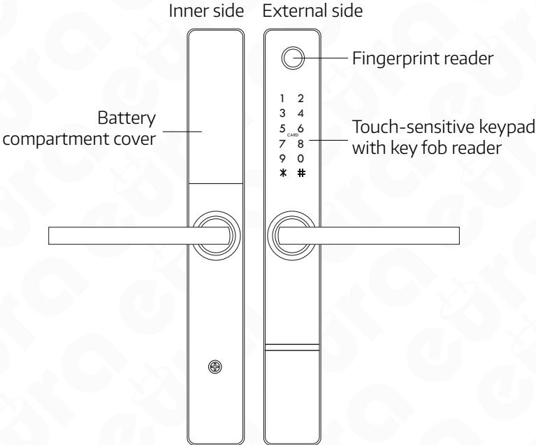
Fig. 2. Construction
