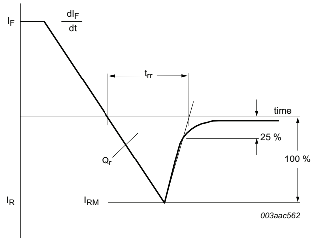
Fig. 7. Reverse recovery definitions; ramp recover
