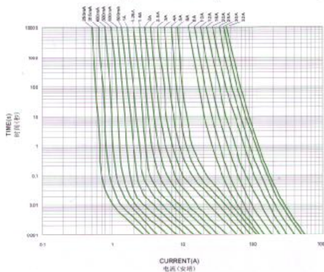
HC10aR AVERAGE I-T CHARACTERISTICS CURVE (FOR REFERENCE)
