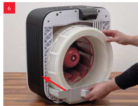
Insert the water tray with the drum into the appliance.
