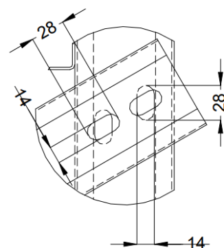
DETAL / DETAIL B SKALA / SCALE 1 : 5
