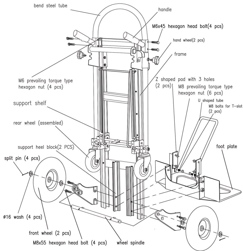
instruction diagram
