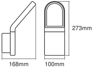
PG ENDURA STYLE Wall (Sensor) MiPRC
