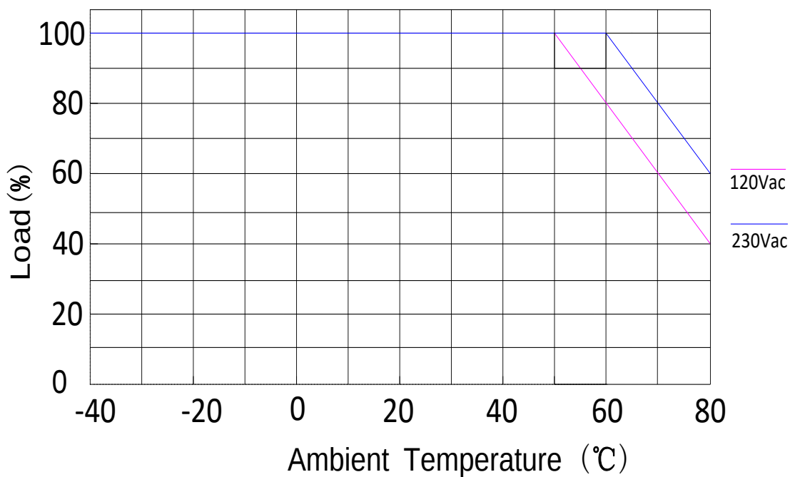
Derating Curve
