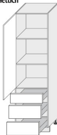
D/14/DP/3A (600/2070/565)
