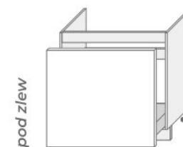
D1ZM 80 ● (800/820/500)
