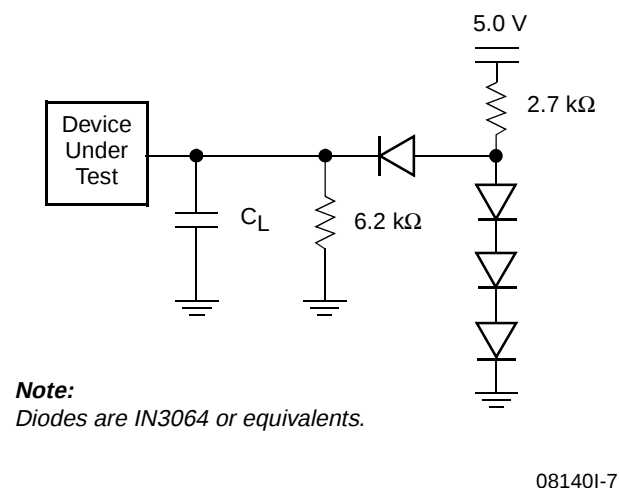
Figure 3. Test Setup
