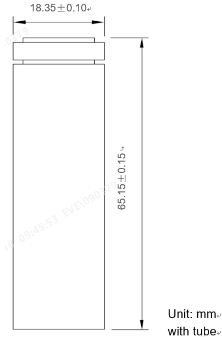
Fig. 1. Outline Dimensions of INR18650/30P
