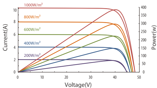
IV Curves of JT385SGh at different irradiances
