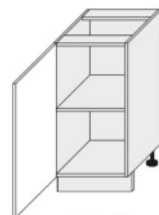
D1D 40 (400/820/500)
