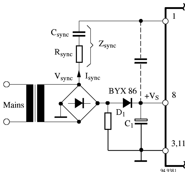
Figure 7. Mains synchronisation
