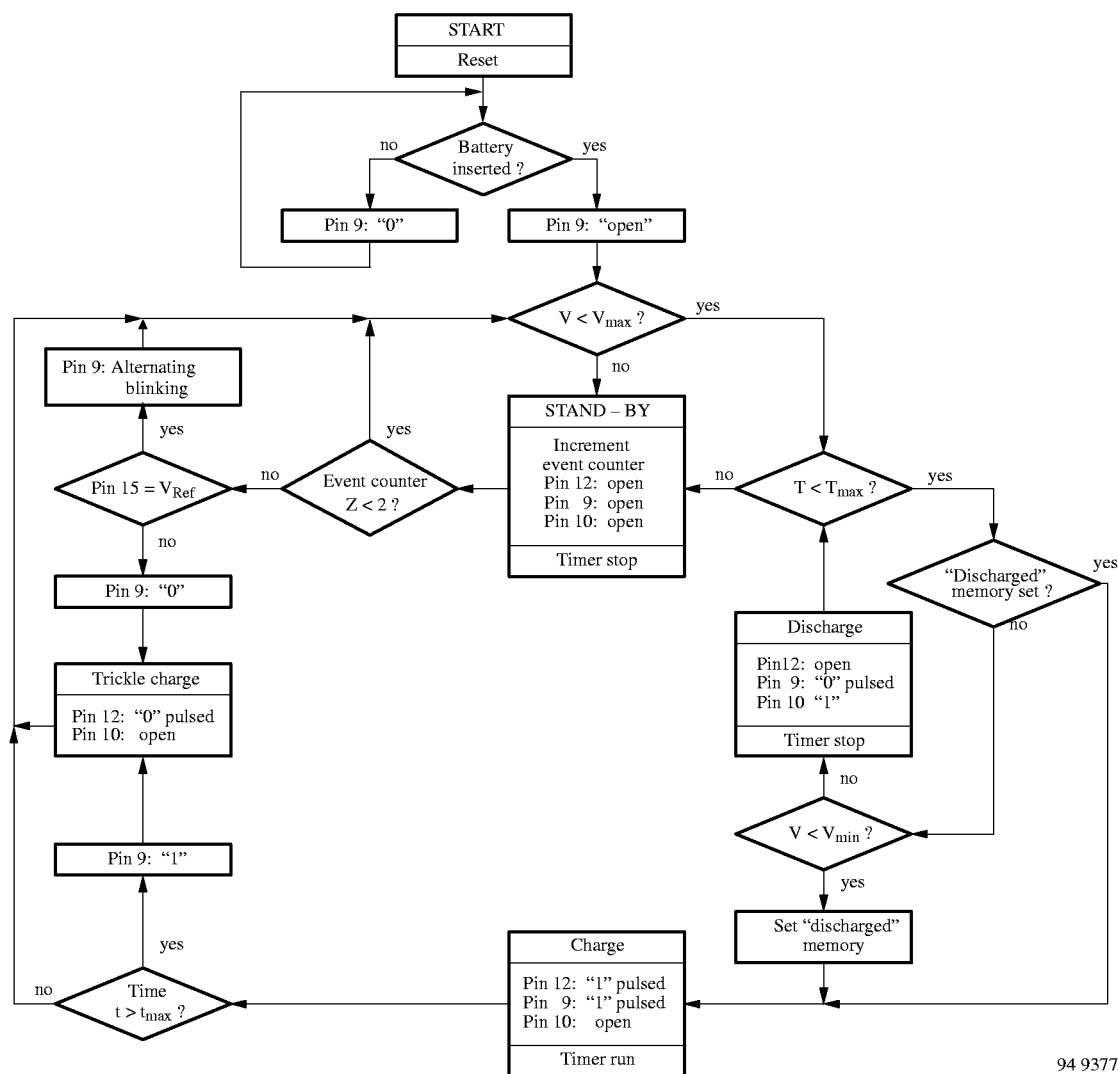
Figure 3. Flow chart
