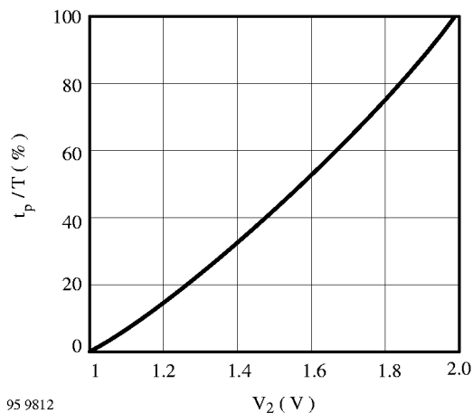
Figure 11. Duty cycle of PWM circuit of figure 9
