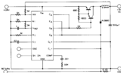
FIGURE 3 - CURRENT LIMITING CIRCUITRY OF THE SG1524
