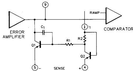
FIGURE 3 - CURRENT LIMITING CIRCUITRY OF THE SG1524
