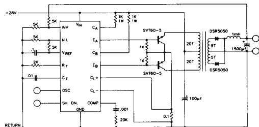
FIGURE 3 - CURRENT LIMITING CIRCUITRY OF THE SG1524
