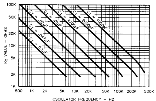
FIGURE 2 - OSCILLATOR FREQUENCY VS. R 1 AND C 1
