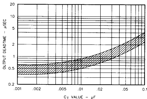
FIGURE 1 - OUTPUT STAGE DEADTIME VS. C_o
