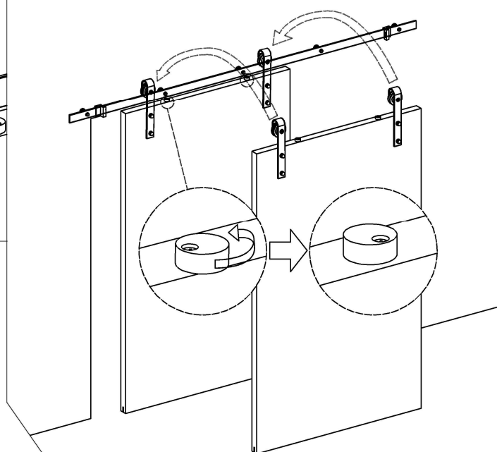
Step6: Install door & fix anti-jumper
