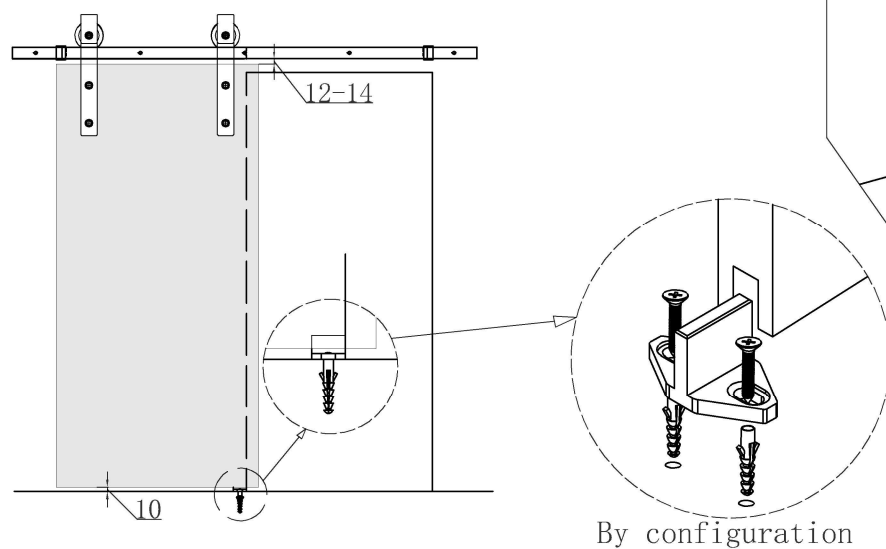
Step7: Install floor guide
