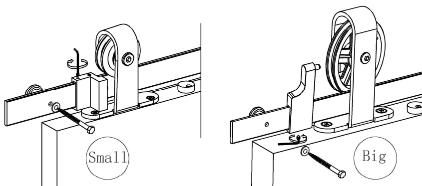
Step7: Install floor guide
