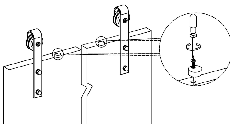
Step6: Install door & fix anti-jumper
