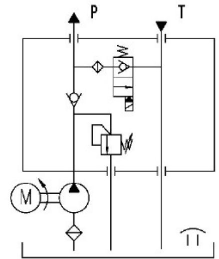
HYDRAULIC CIRCUIT
