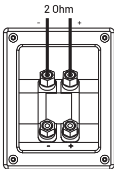
MAD B1-212 parallel connection (normal)
