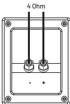
MAD B1-112 connection
