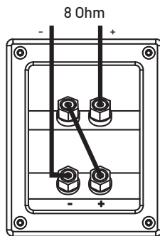
MAD B1-212 serial connection
