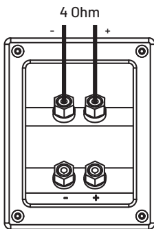
MAD B1-212 singular connection
