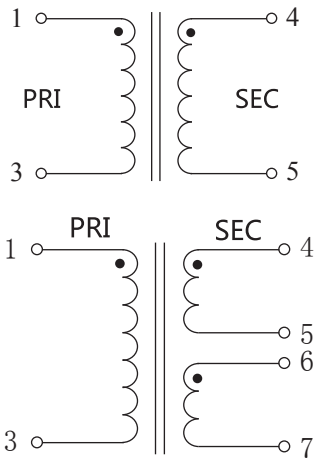
Schematic Diagram
