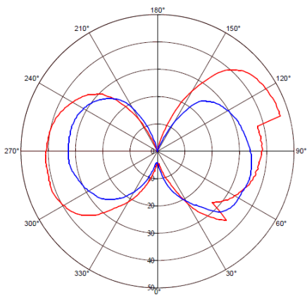
Photometric Diagram
