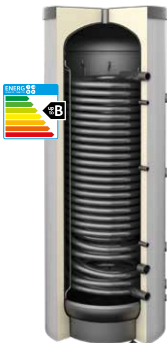
pic. 32 SG(B) with the maximum size spiral coil
