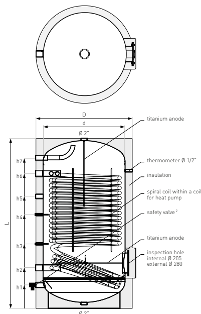
scheme - SGW(S) Maxi 800-1000
