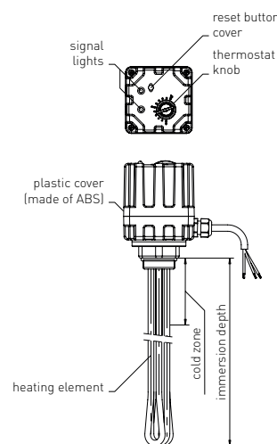
scheme - 4,5-9 kW electrical set with a plug
