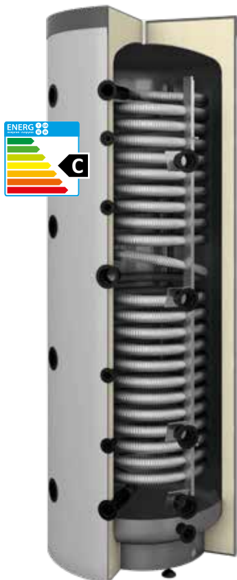
pic. 28 SG(K) Multi-Inox
