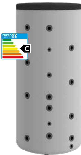
pic. 36 SG(B) with two maximum size spiral coils
