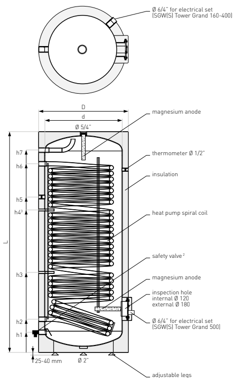
scheme - SGW(S) Tower Grand
