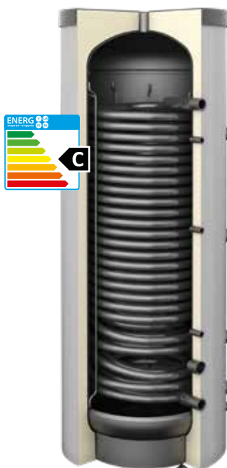
pic. 34 SG(B) with the maximum size spiral coil
