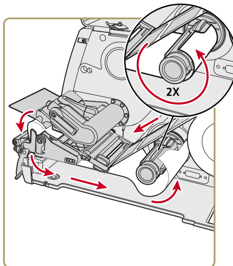
Route the Liner Around a Collapsible Core (PM43, PM43c)
