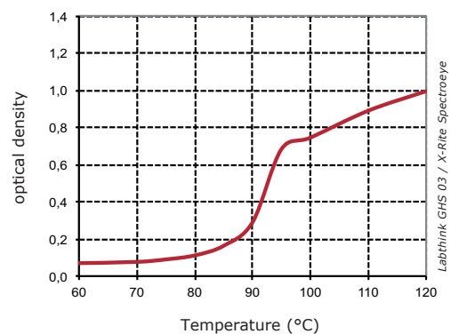
Static Sensitivity
