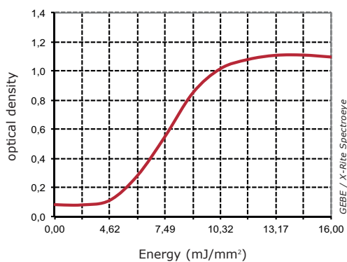
Dynamic Sensitivity
