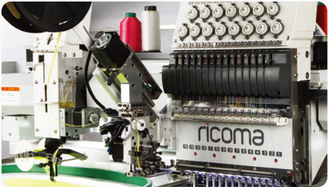
Cording Device (CD-E) Easily create an embroidery effect with the cording device, which lays cord on fabric and attaches the cord with transparent zigzag
