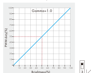
Linear dimming curve
