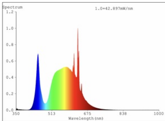
LED GX53 83 120
