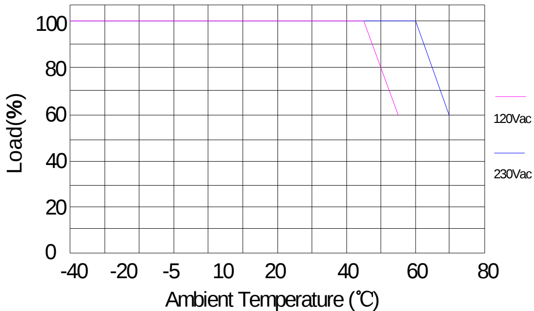
Derating Curve
