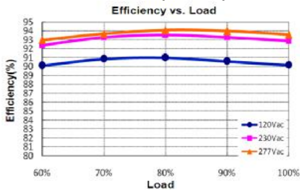
X6-200Y096 (Io=2.10A)
