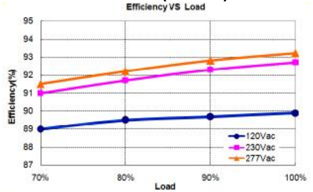
X6-200Y143 (Io=2.10A)
