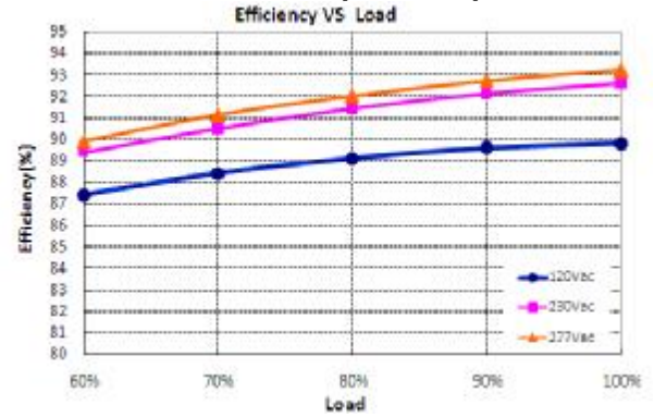
X6-200Y096 (Io=3.00A)
