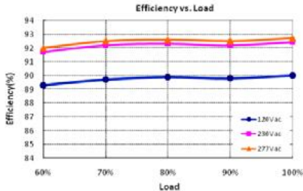
X6-200Y286 (Io=0.70A)
