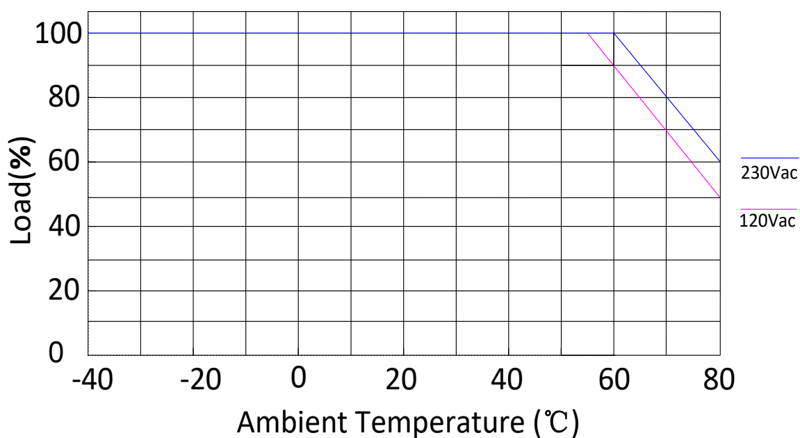
Derating Curve
