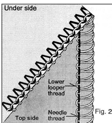
Lower looper thread pulled to under side
