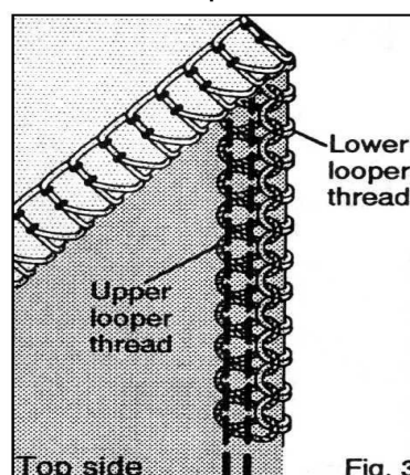
Lower looper thread pulled to top side
