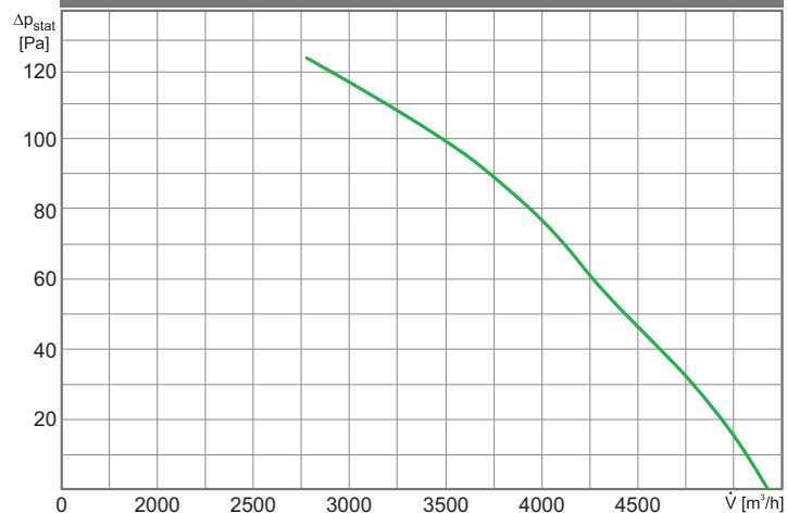
WAX 450/N/4/5100S
