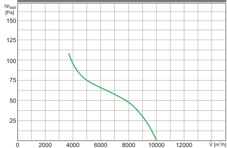
WAX 630/W/6/9500S
