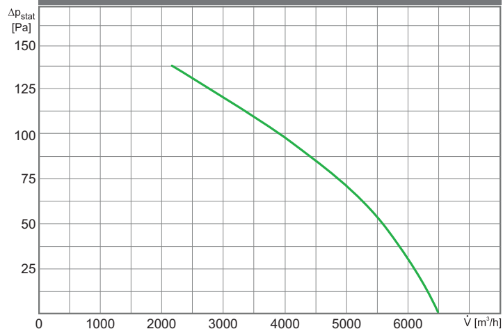
WAX 500/W/4/6500S
