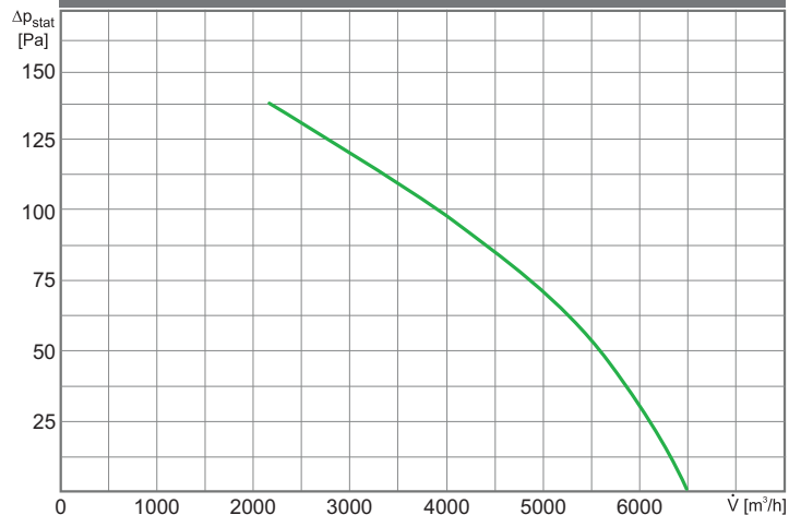
WAX 500/N/4/6500S
