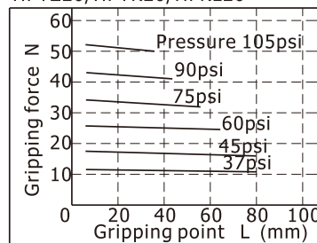
HFTZ40/HFTK40
