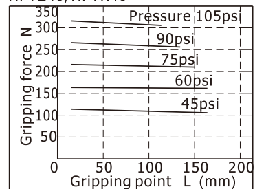
HFTZ40/HFTK40
