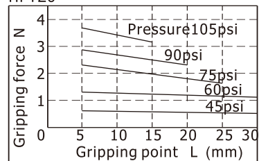
HFTZ20/HFTK20/HFKL20
