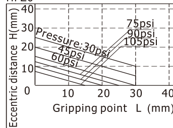
HFZ20/HFK20/HFKL20
