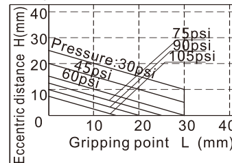
HFZ20/HFK20/HFKL20
