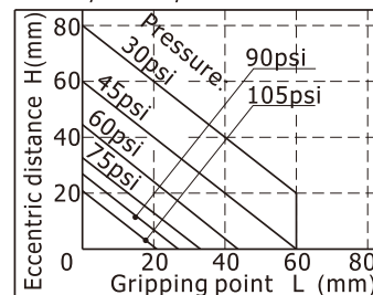
HFZ40/HFK40
