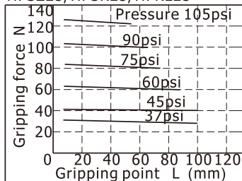
HFSZ25/HFSK25/HFKL25
