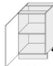
D1D 50 (500/820/500)
