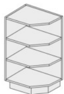
D6 30 (300/820/500)
