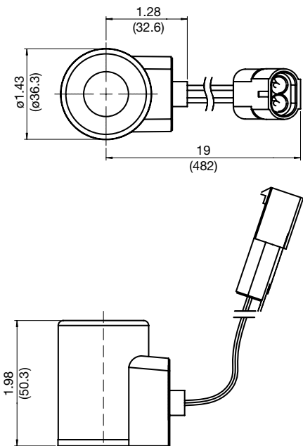
WeatherPak™ 12010973
