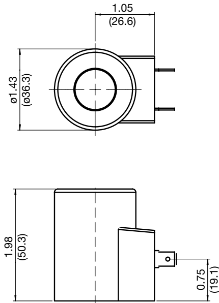
Dual 1/4" Spades
