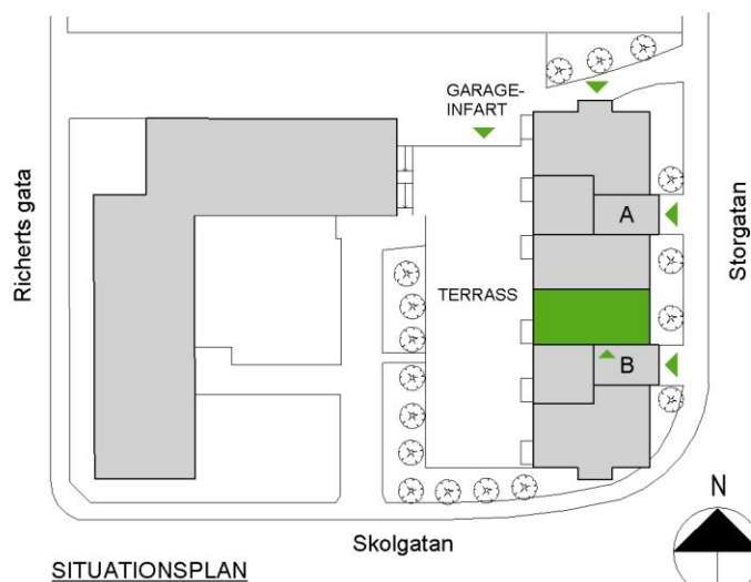
SITUATIONSPLAN
