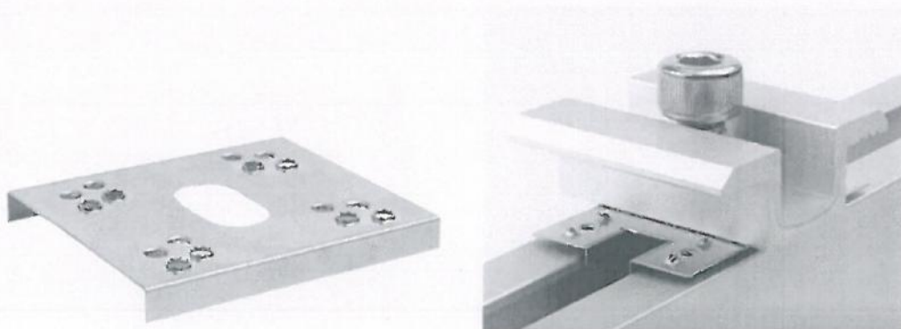
Fig. 5-10 Double spine ground gasket and installation diagram
