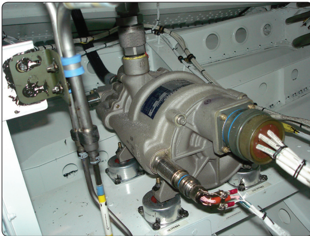
Figure 12-22. Electrically-driven pump.
