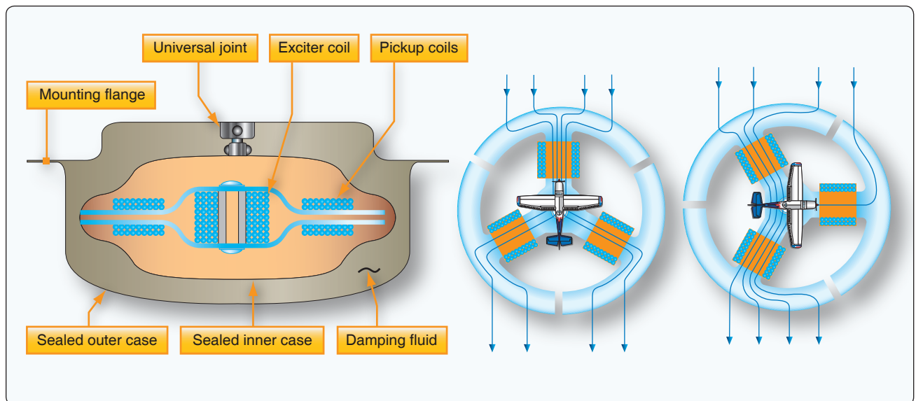
Figure 10-83. As the aircraft turns in the earth's magnetic field, the lines of flux flow lines vary through the permeable core of flux gate, creating variable voltages at the three pickoffs.
