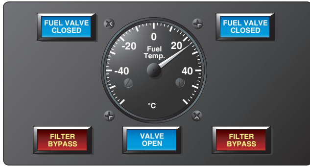
Figure 14-64. A Boeing 737 cockpit fuel panel showing illuminated valve position indicators and fuel filter bypass lights. The fuel temperature in tank No.1 is also indicated.
