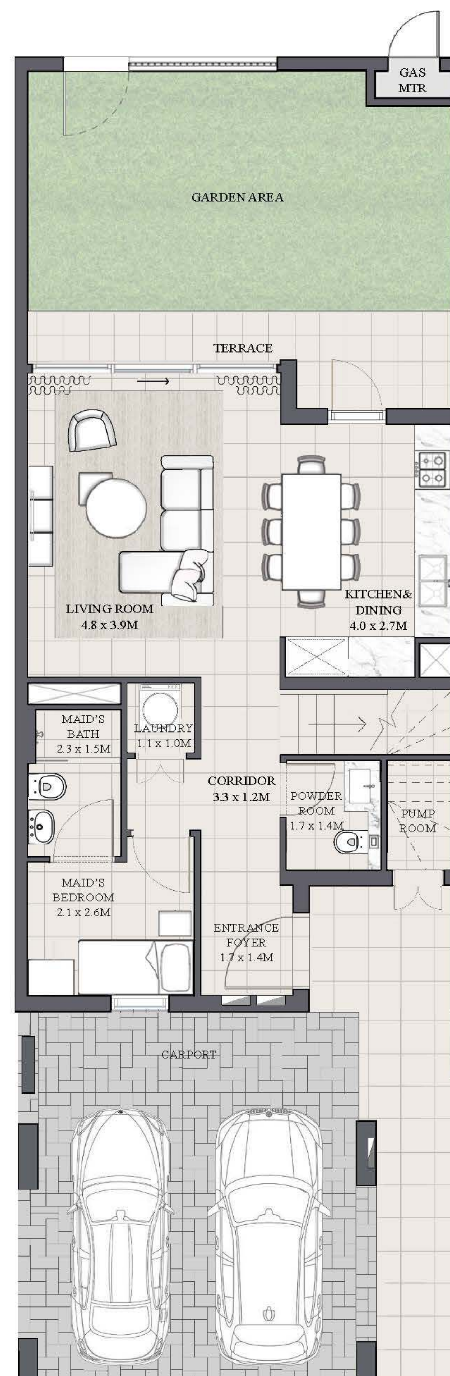
GROUND FLOOR
