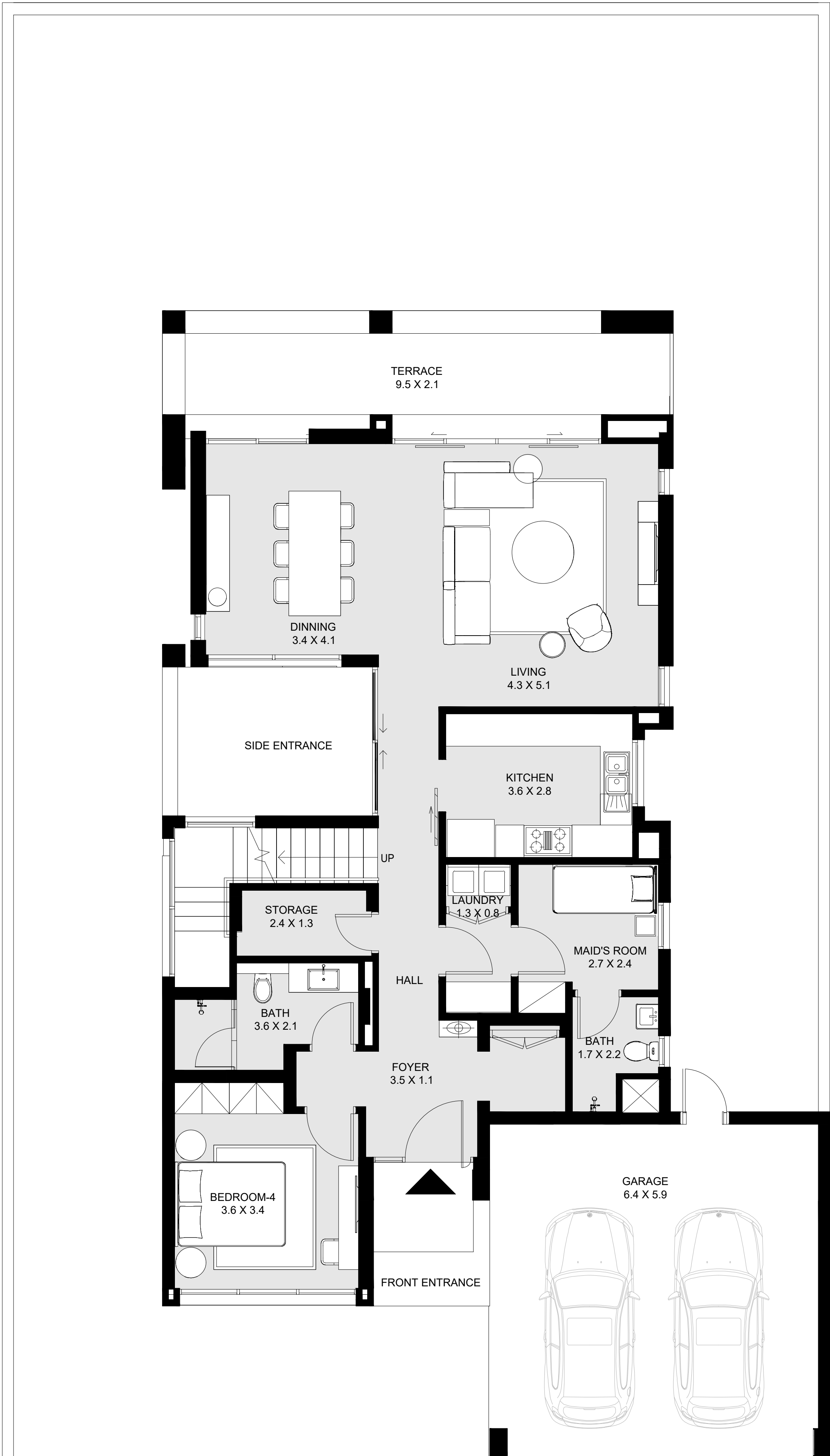
GROUND FLOOR
