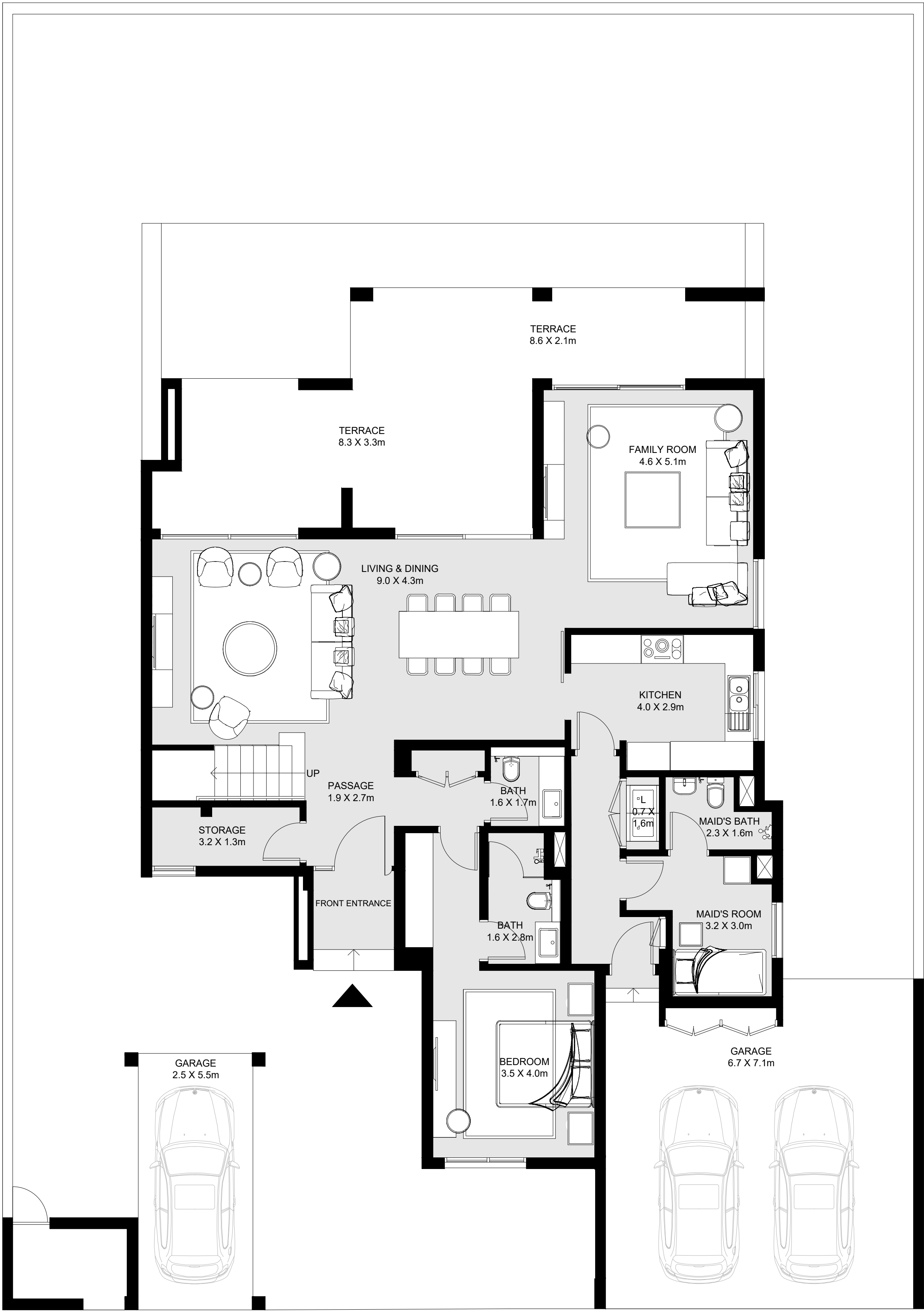
GROUND FLOOR
