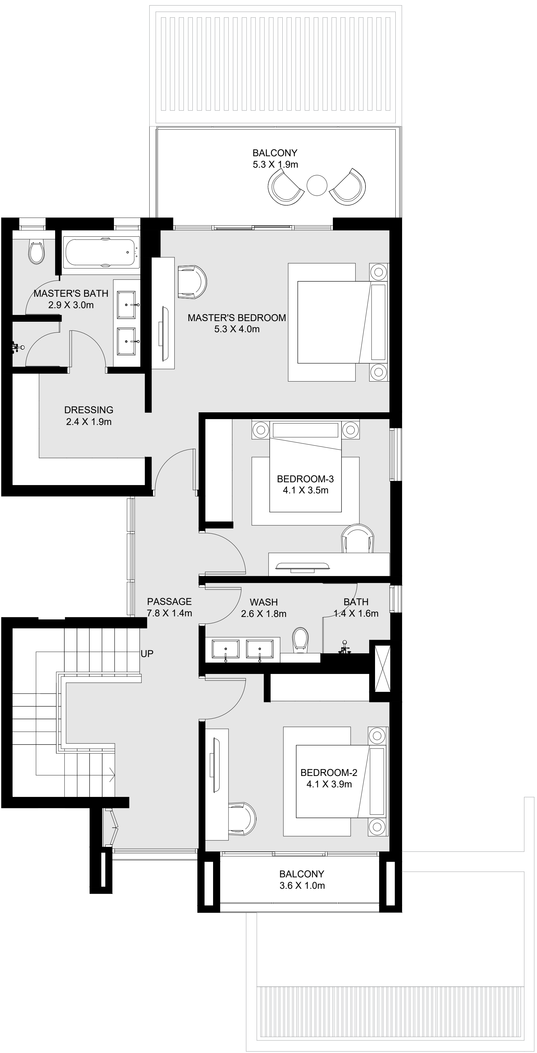
FIRST FLOOR
