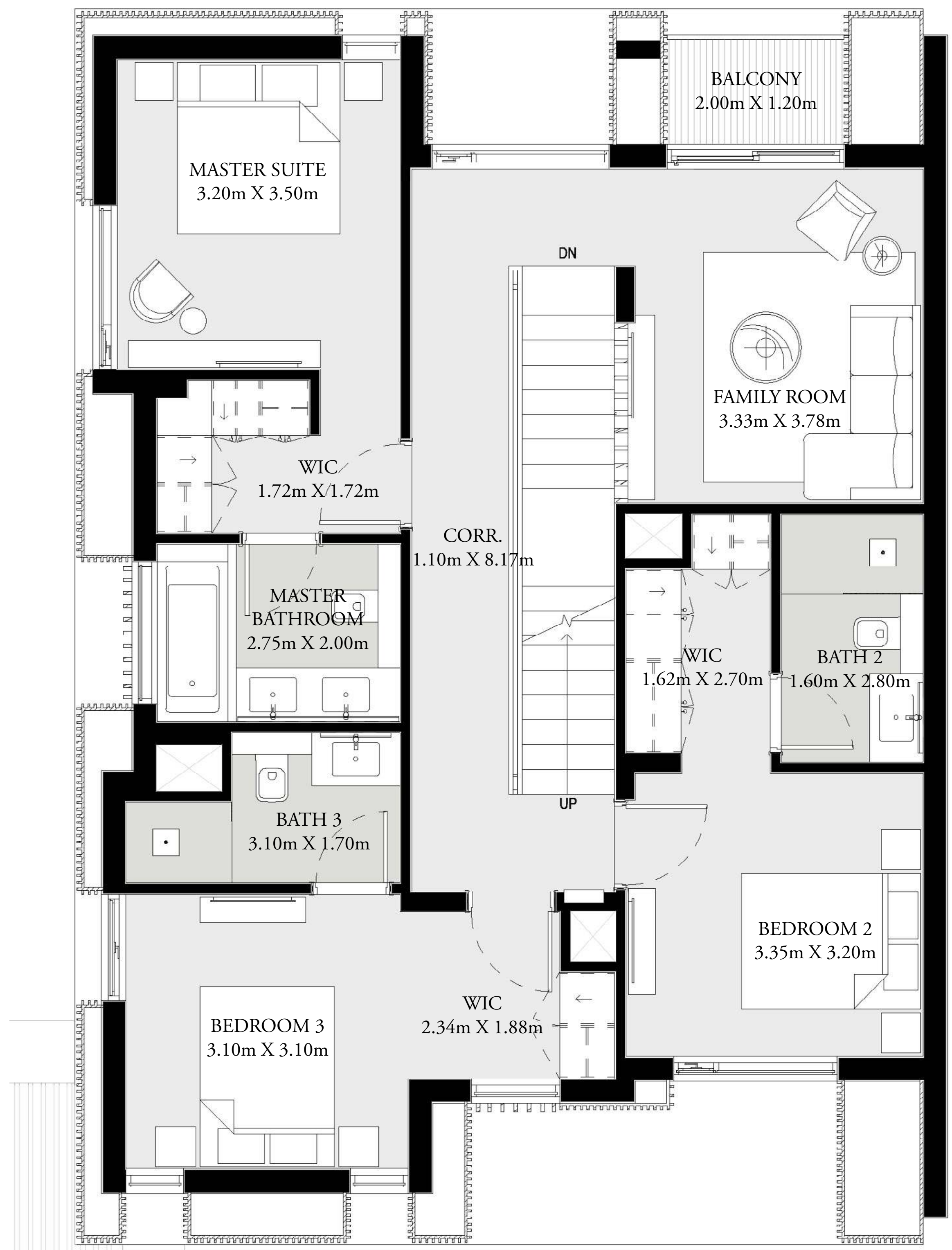
FIRST FLOOR
