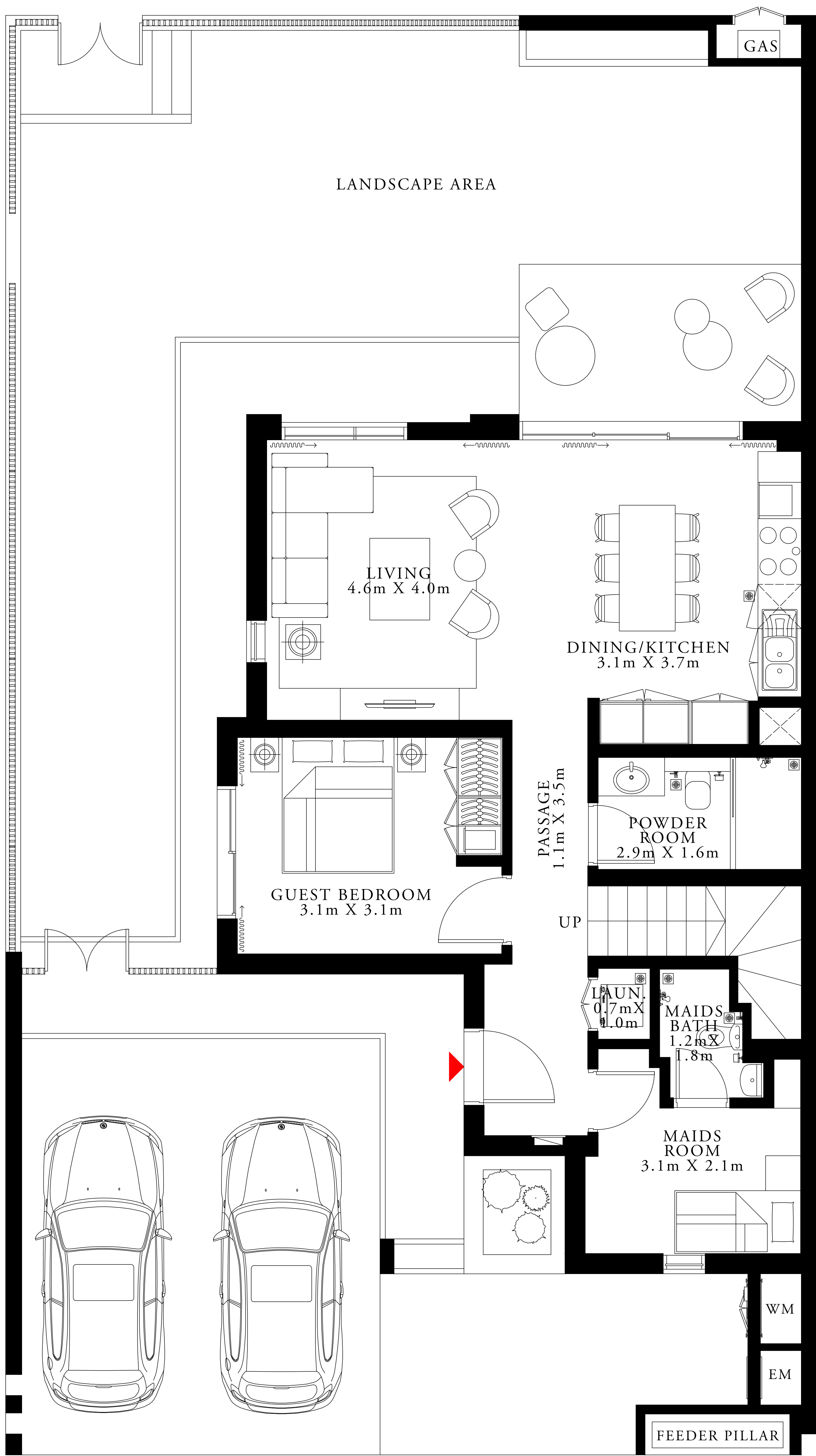
GROUND FLOOR
